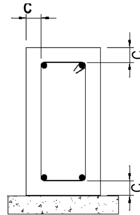
GRADE BEAM
